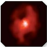
MS 0735.6+7421: A cluster of galaxies about 2.6 billion light years from Earth.
