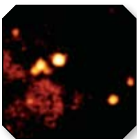
M82: A starburst galaxy (central region) about 11 million light years from Earth.
