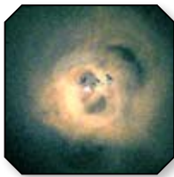
PERSEUS CLUSTER: A galaxy cluster about 250 million light years from Earth.
