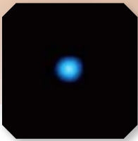
RX J1242-11: A galaxy about 700 million light years from Earth.
