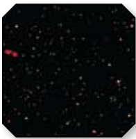
LOCKMAN HOLE: A region of the sky away from the Galactic plane that provides a relatively clear view to objects ranging from nearly a billion to over 12 billion light years from Earth.
